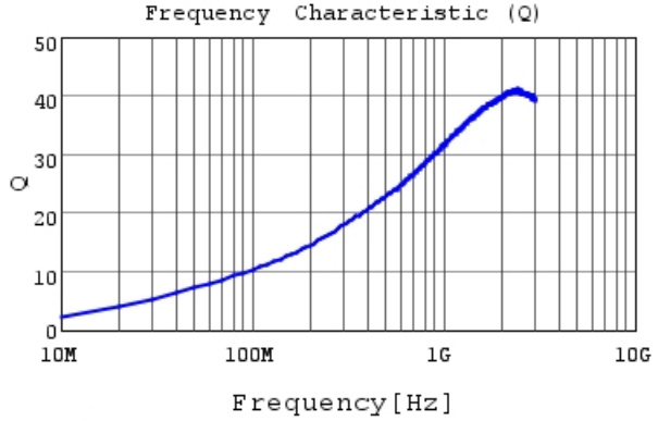
LQP03TQ8N2J02 Q
