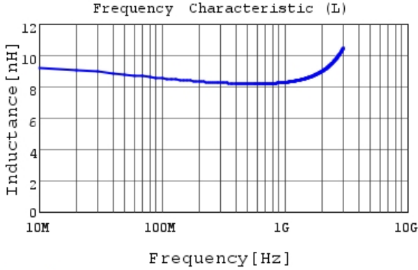
LQP03TQ8N2J02 L
