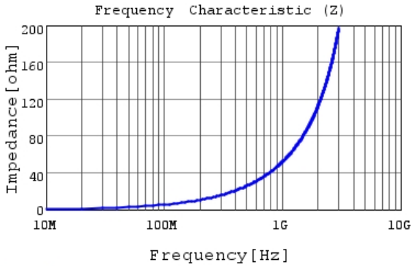
LQP03TQ8N2J02 |Z|
