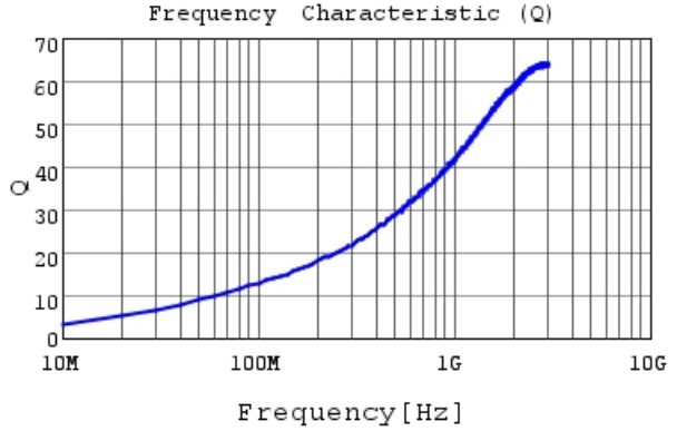
LQG15HN2N2B02 Q
