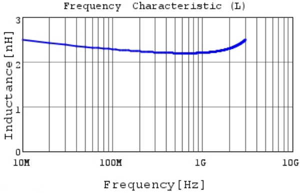
LQG15HN2N2B02 L
