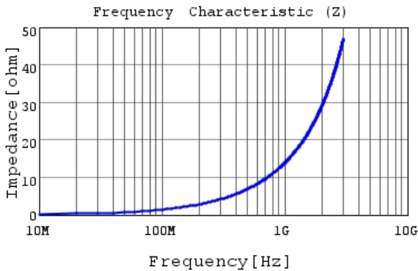
LQG15HN2N2B02 |Z|
