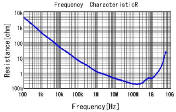
GRM188R71H182KA01 R DCOV, 25degC
