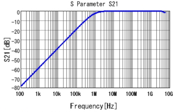
GRM188R71H182KA01 S21 DC0V, 25degC
