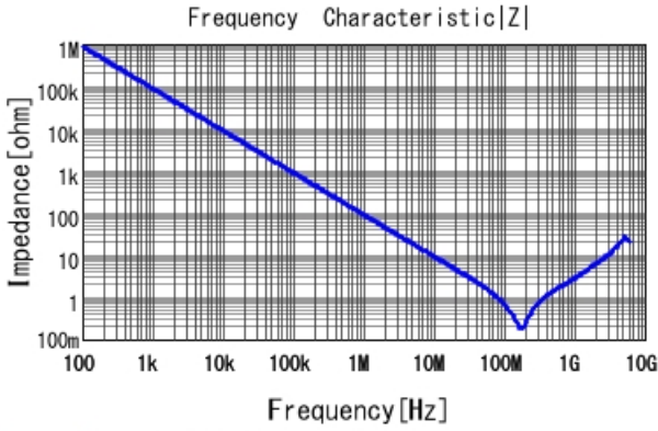
GRM188R71H182KA01 |Z| DCOV, 25degC
