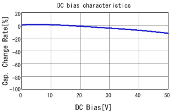
GRM188R71H182KA01 C-DC bias capchange, 25.0degC, A
