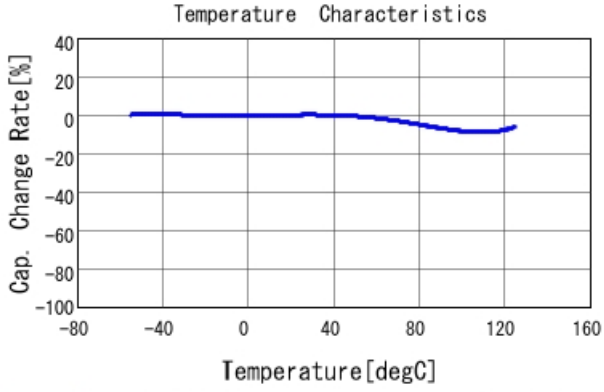
GRM188R71H182KA01 C-Temp. capchange, DC0.0V, AC1.C
