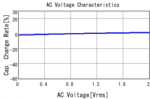
GRM188R71H182KA01 C-AC Voltage capchange, DCOV, 25
