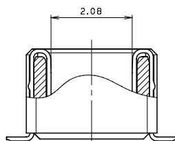
SECT. S-S
