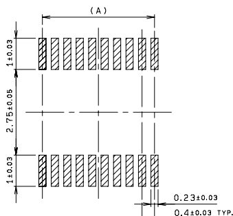
MOUNTING LAYOUT
