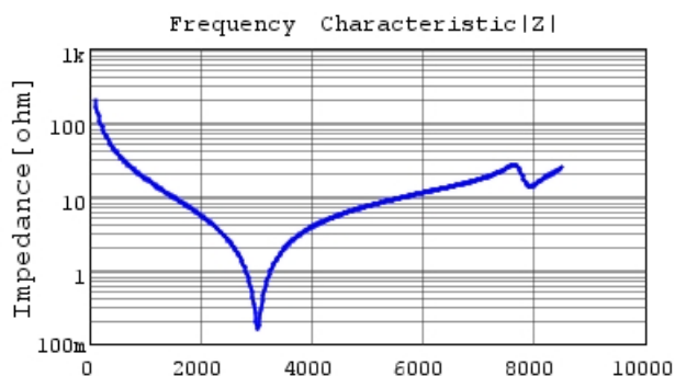
GCQ1555C1H8R2CB01 |Z| DCOV,25degC
