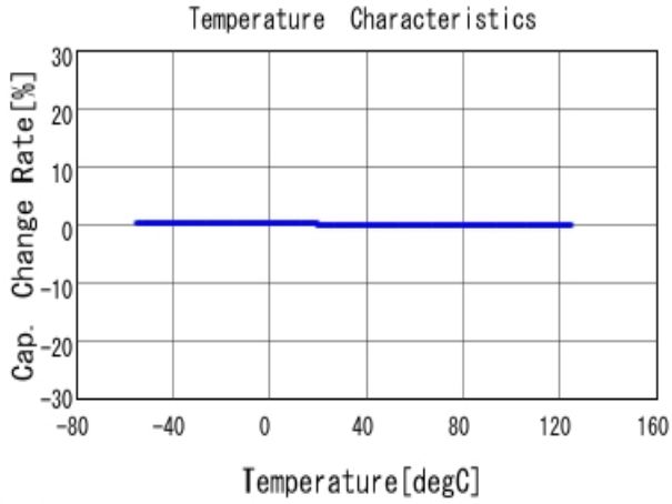
■ GRM1882C1E821JA01 C-Temp. capchange, DCOV, AC1Vrms
