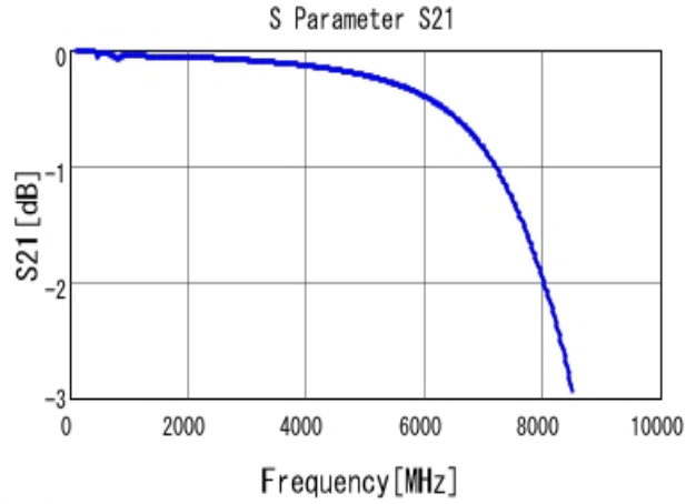
■ GRM1882C1E821JA01 S21 DCOV, 20degC
