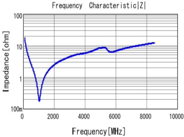
■ GRM0332C2A910JA01 |Z| DC0V, 20degC
