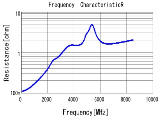
■ GRM0332C2A910JA01 R DC0V, 20degC
