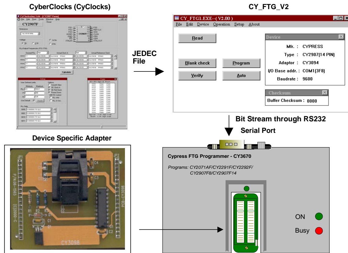
Figure 1-1. Programming Procedure
