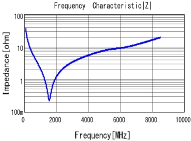
■ GRM0332C1H430JA01 |Z| DCOV, 20degC
