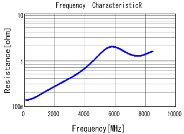
■ GRM0332C1H430JA01 R DCOV, 20degC
