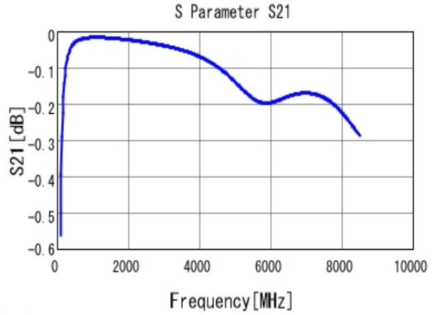
■ GRM0332C1H430JA01 S21 DCOV, 20degC
