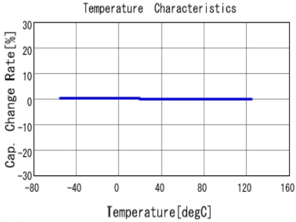
■ GRM0332C1H430JA01 C-Temp. capchange, DCOV, AC1Vrms
