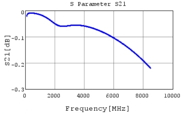
GRM0332C1E271JA01 S21 DCOV, 20degC
