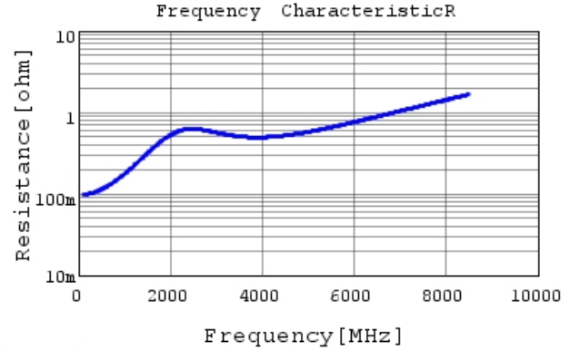
GRM0332C1E271JA01 R DCOV, 20degC
