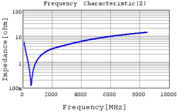
GRM0332C1E271JA01 |Z| DCOV, 20degC
