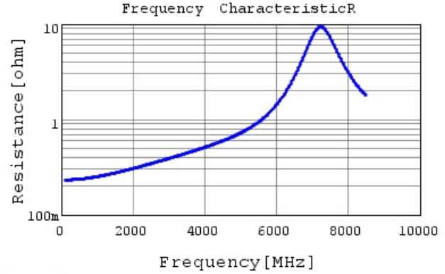
GCM1555C1H5R6CA16 R DC0V, 25degC
