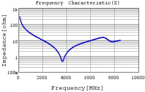
GCM1555C1H5R6CA16 |Z| DC0V, 25degC
