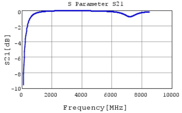
GCM1555C1H5R6CA16 S21 DCOV, 25degC
