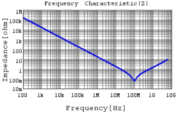
GRM033B31C103MA12 |Z| DCOV, 20degC
