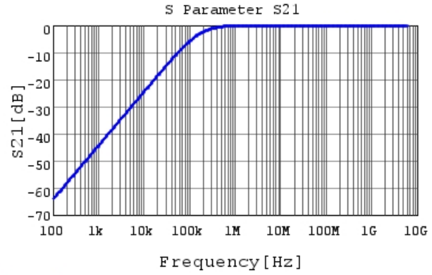
GRM033B31C103MA12 S21 DC0V,20degC
