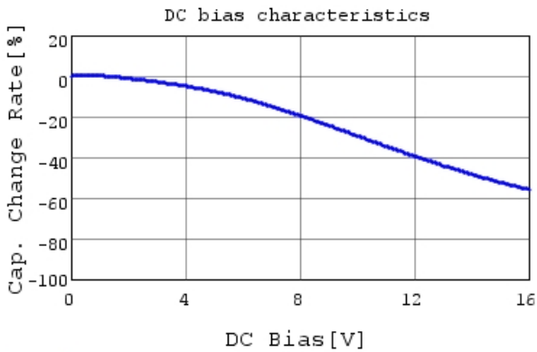
GRM033B31C103MA12 C-DC bias capchange, 20.0c
