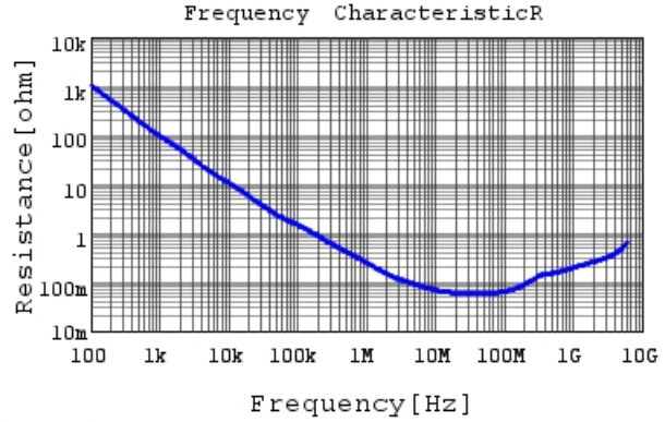
GRM033B31C103MA12 R DCOV, 20degC
