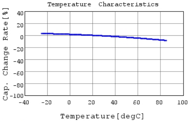
GRM033B31C103MA12 C-Temp. capchange, DC0.0V,
