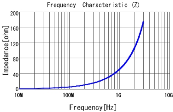
LQW03AW8N2J00 |Z|
