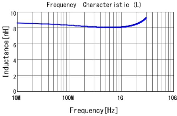
LQW03AW8N2J00 L
