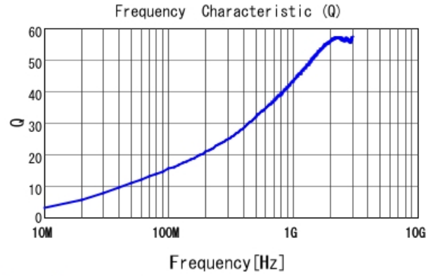
LQW03AW8N2J00 Q
