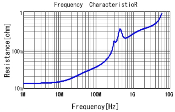
GRM1557U1A332JA01 R DCOV, 25degC
