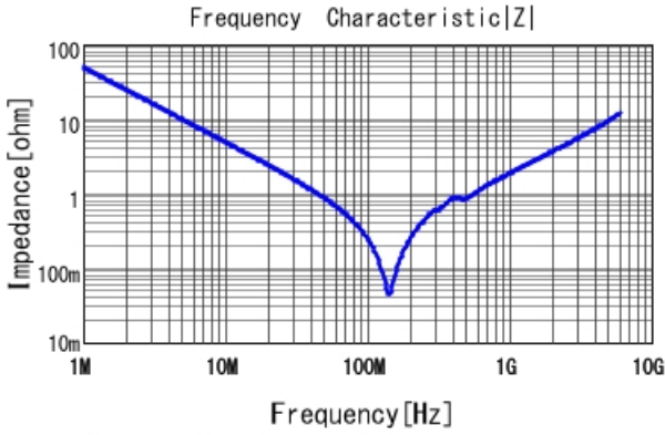
GRM1557U1A332JA01 |Z| DCOV, 25degC
