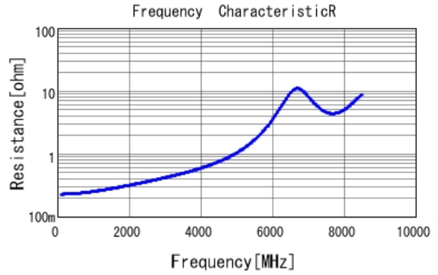
GCM1555C1H6R8DA16 R DCOV, 25degC
