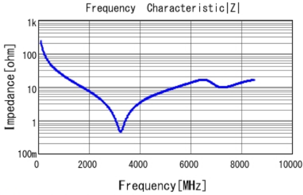
GCM1555C1H6R8DA16 |Z| DCOV, 25degC
