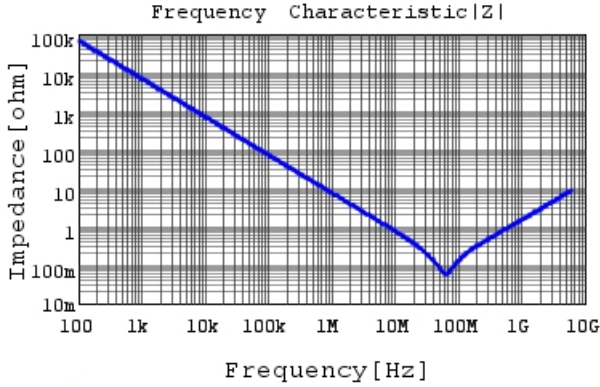
GRM033B31A273KE84 |Z| DCOV, 20degC
