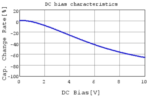
GRM033B31A273KE84 C-DC bias capchange, 20.0c
