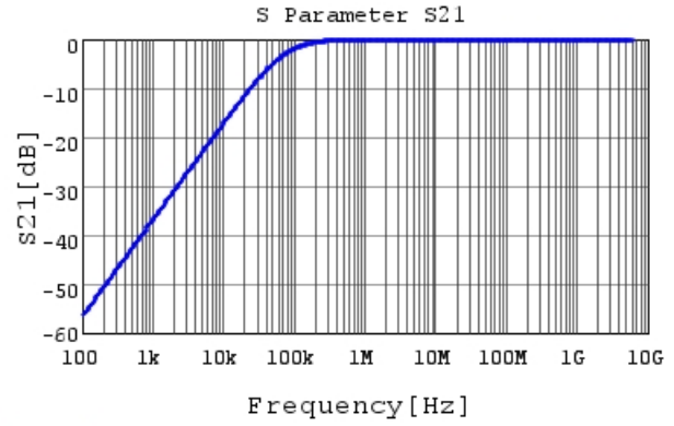
GRM033B31A273KE84 S21 DC0V, 20degC
