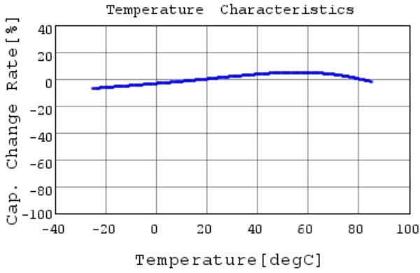
GRM033B31A273KE84 C-Temp. capchange, DC0.0V,
