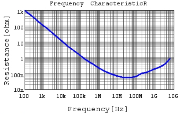
GRM033B31A273KE84 R DCOV, 20degC
