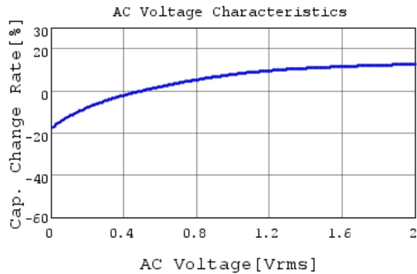
GRM033B31A273KE84 C-AC Voltage capchange, Dc
