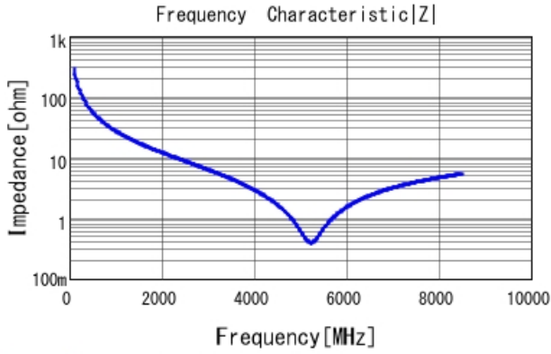
GRM0225C1E5R6DA03 |Z| DCOV, 25degC
