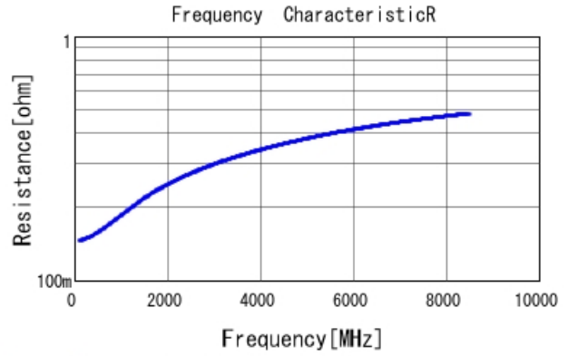
GRM0225C1E5R6DA03 R DCOV, 25degC
