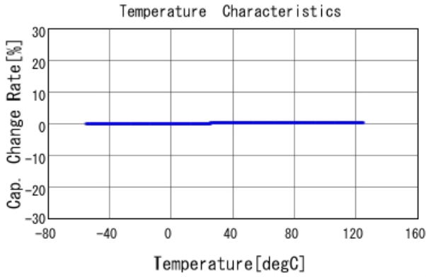
GRM0225C1E5R6DA03 C-Temp. capchange, DC0V, AC1Vrms
