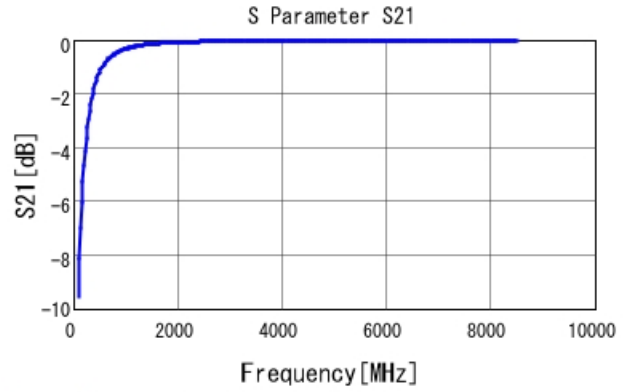
GRM0225C1E5R6DA03 S21 DC0V, 25degC
