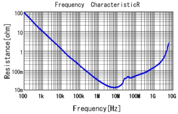
GRM188R61H474MA12 R DCOV, 25degC
