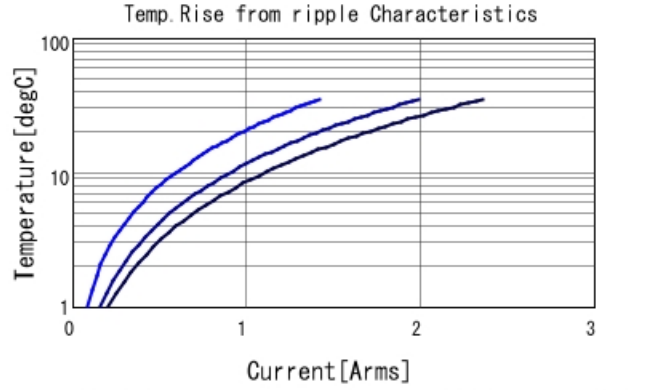
GRM188R61H474MA12 Temp. rise — 200kHz — 500
