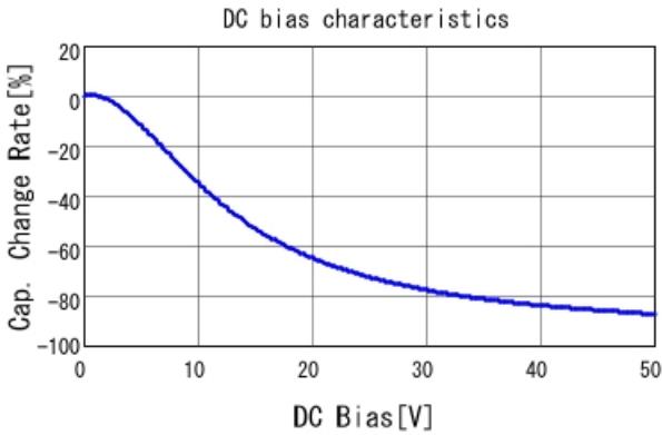
GRM188R61H474MA12 C-DC bias capchange, 25.0degC, A
