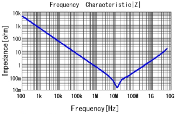
GRM188R61H474MA12 |Z| DCOV, 25degC
