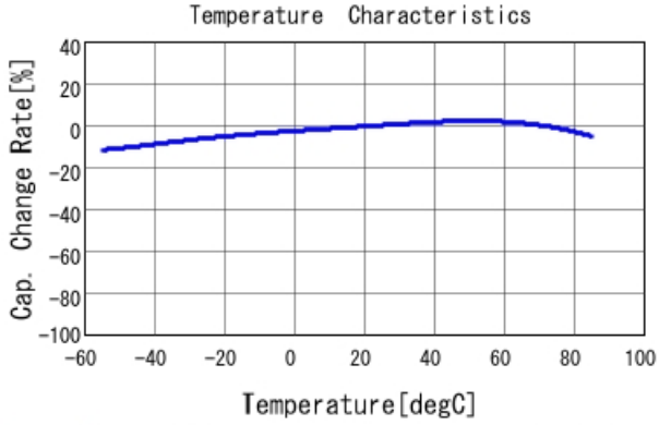
GRM188R61H474MA12 C-Temp. capchange, DC0.0V, AC1.5
