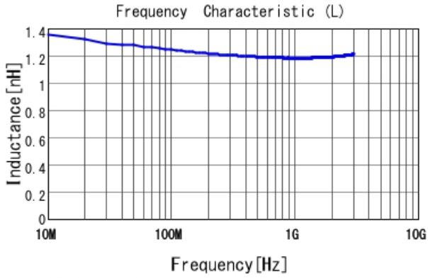
LQP03TN1N2CZ2 L
