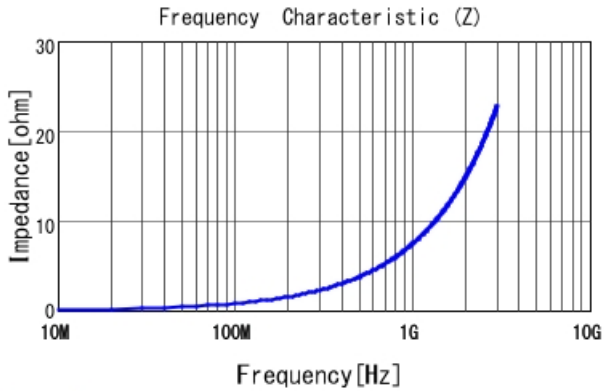
LQP03TN1N2CZ2 |Z|
