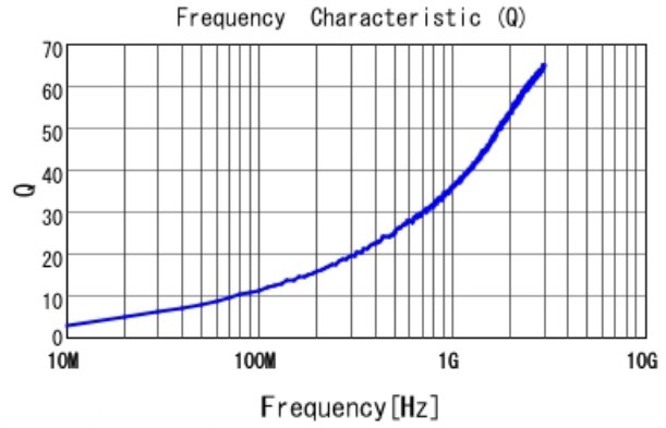
LQP03TN1N2CZ2 Q
