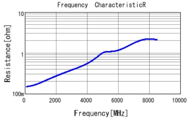
■ GRM0335C2A240JA01 R DCOV, 25degC
