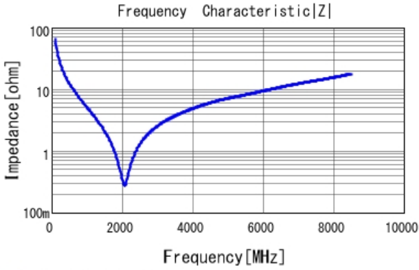
■ GRM0335C2A240JA01 |Z| DCOV, 25degC
