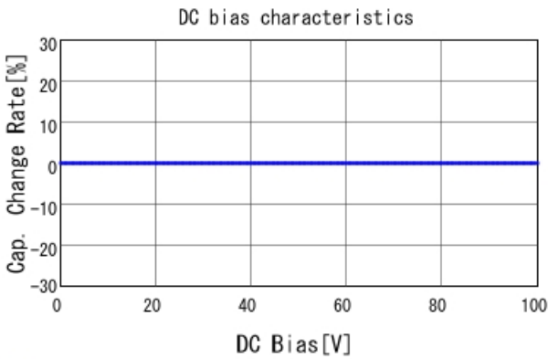
■ GRM0335C2A240JA01 C-DC bias capchange, 25.0degC, AC1V
