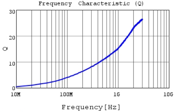
LQP02TN2N7C02 Q
