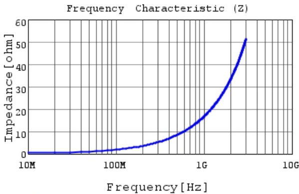
LQP02TN2N7C02 |Z|
