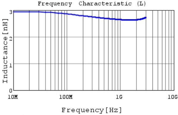
LQP02TN2N7C02 L
