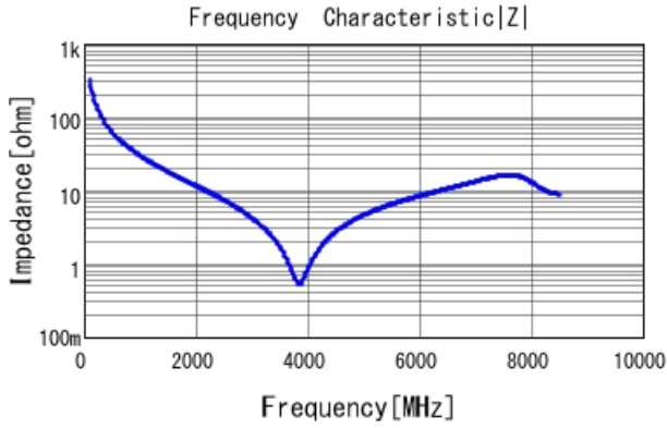
GRM1555C2A5R0CA01 |Z| DCOV, 25degC
