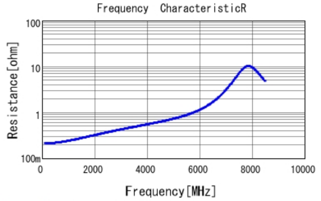
GRM1555C2A5R0CA01 R DCOV, 25degC
