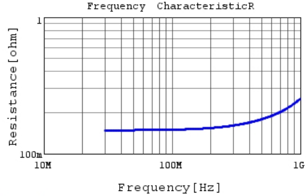
RDE5C1H101J0P1H03B R DC0V, 25degC
