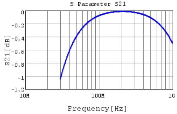
RDE5C1H101J0P1H03B S21 DCOV, 25degC
