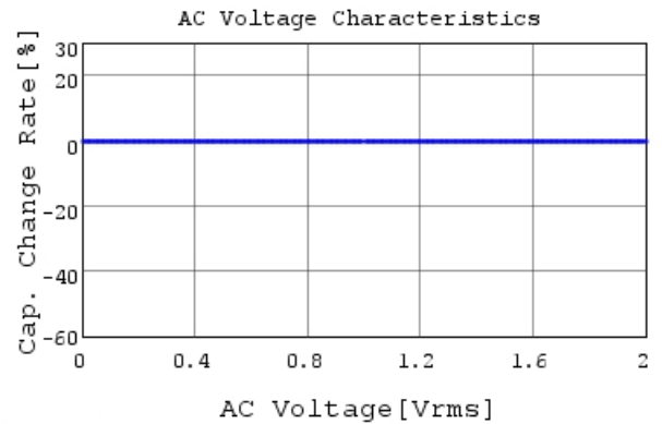
RDE5C1H101J0P1H03B C-AC Voltage capchange, I
