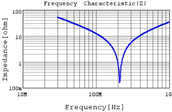
RDE5C1H101J0P1H03B |Z| DC0V, 25degC
