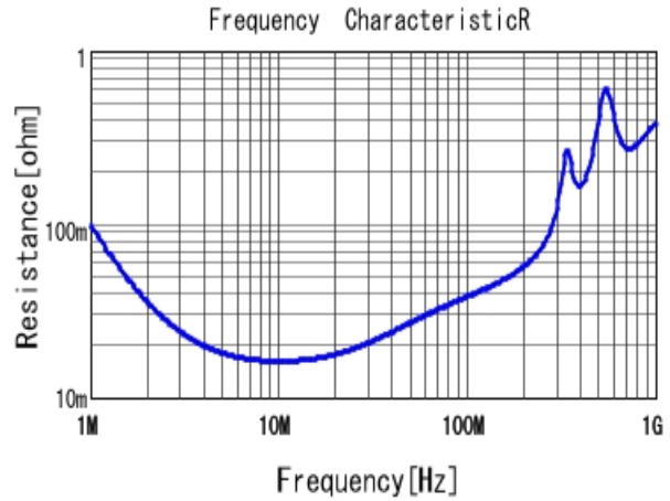
GCM21A5C2E222JX01 R DC0V, 25degC
