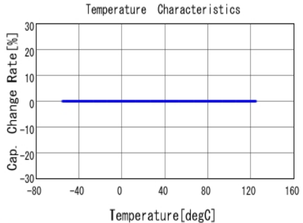
GCM21A5C2E222JX01 C-Temp. capchange, DC0V, AC1Vrms
