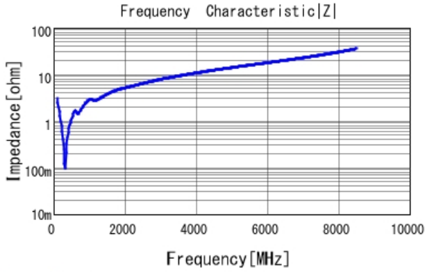
GRM1885C2A471JA01 |Z| DCOV, 25degC
