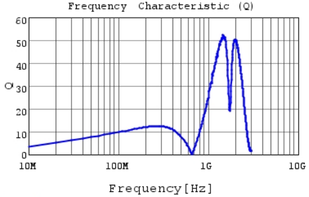
LQG15HSR22J02 Q
