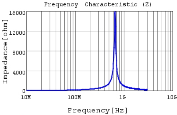
LQG15HSR22J02 |Z|
