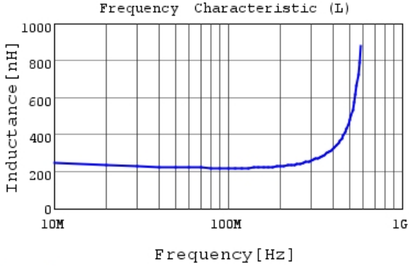
LQG15HSR22J02 L
