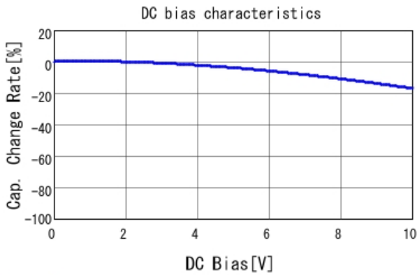
GRM31CR71A475KA01 C-DC bias capchange, 25.0degC, A
