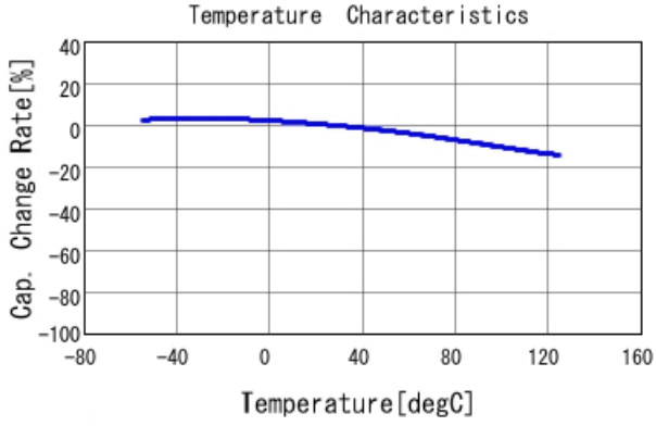
GRM31CR71A475KA01 C-Temp. capchange, DC0.0V, AC1.C
