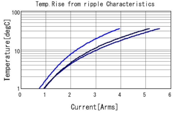
GRM31CR71A475KA01 Temp. rise — 100kHz — 500
