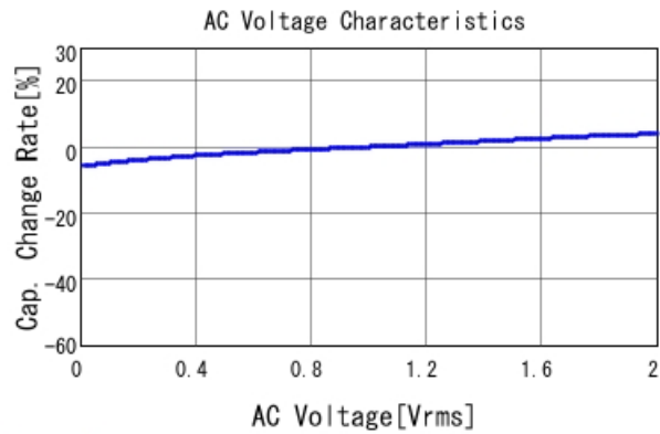
GRM31CR71A475KA01 C-AC Voltage capchange, DCOV, 25
