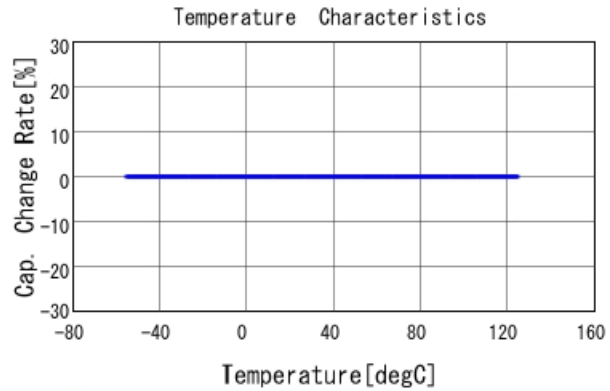
GCM32D5C2J183JX01 C-Temp. capchange, DCOV, AC1Vrms
