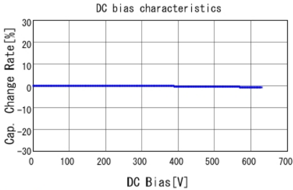
GCM32D5C2J183JX01 C-DC bias capchange, 25.0degC, A
