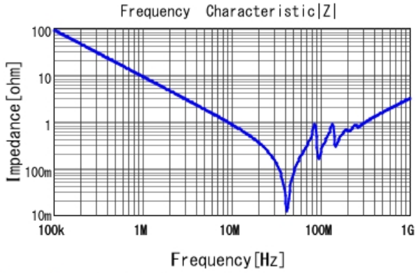
GCM32D5C2J183JX01 |Z| DCOV, 25degC
