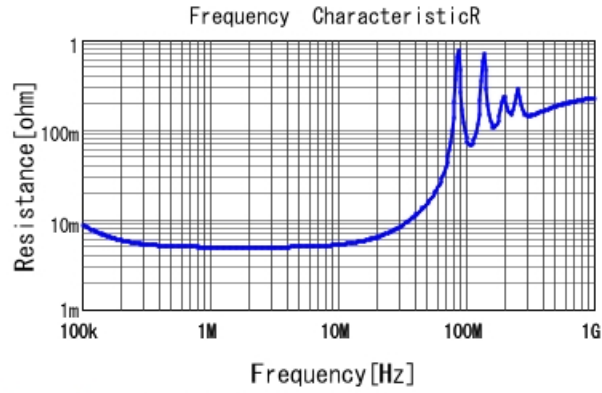
GCM32D5C2J183JX01 R DCOV, 25degC
