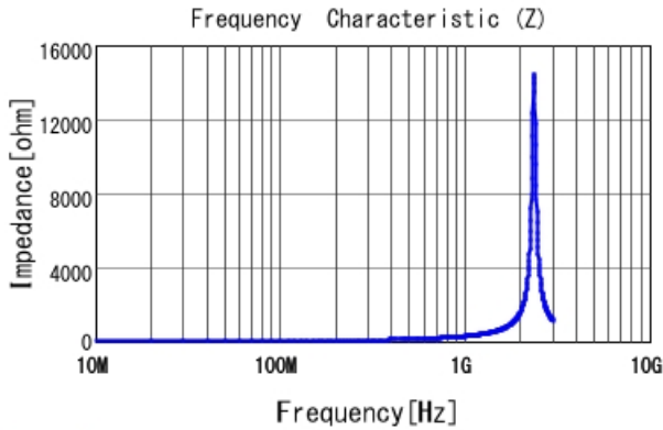
LQP03TN39NJZ2 |Z|
