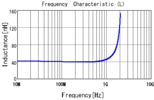
LQP03TN39NJZ2 L
