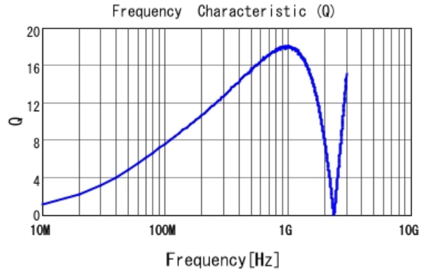
LQP03TN39NJZ2 Q
