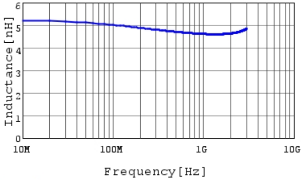
Frequency Characteristic (L)
