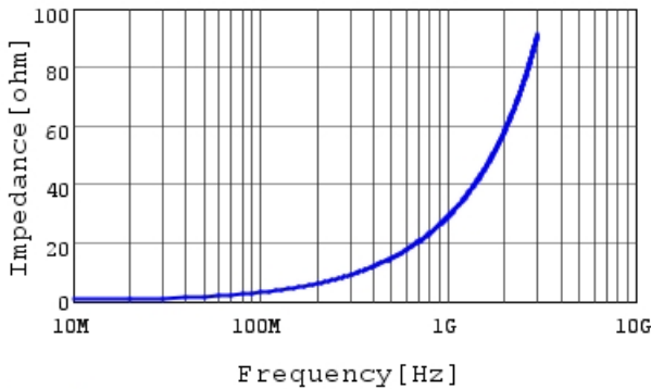
Frequency Characteristic (Z)
