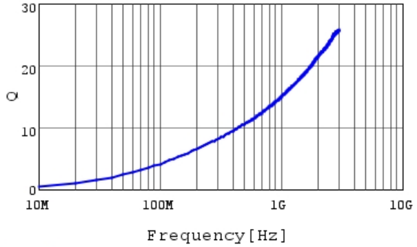
Frequency Characteristic (Q)
