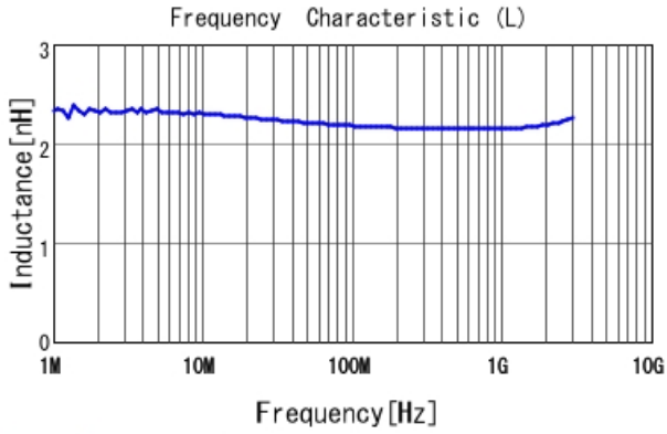
LQW15AN2N2D80 L
