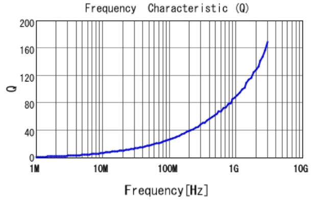
LQW15AN2N2D80 Q
