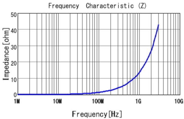
LQW15AN2N2D80 |Z|
