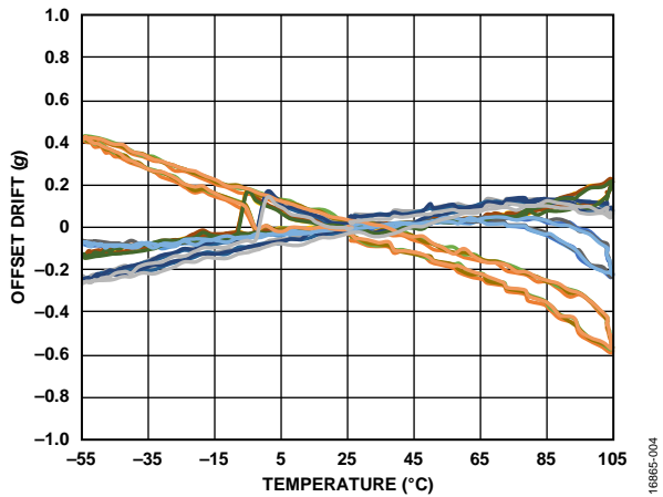
Figure 4. Y-Axis Offset Drift, 15 Devices Soldered to PCB, V_S = 2.5\text{ V}
