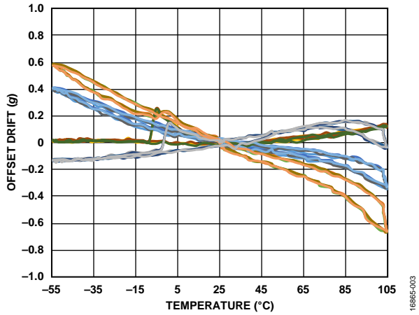
Figure 3. X-Axis Offset Drift, 15 Devices Soldered to PCB, V_S = 2.5\text{ V}
