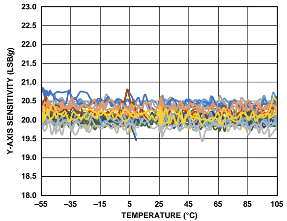
Figure 7. Y-Axis Sensitivity vs. Temperature, 15 Devices Soldered to PCB, V_S = 2.5\text{ V}
