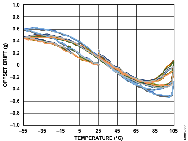
Figure 5. Z-Axis Offset Drift, 15 Devices Soldered to PCB, V_S = 2.5\text{ V}
