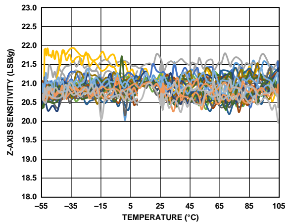
Figure 8. Z-Axis Sensitivity vs. Temperature, 15 Devices Soldered to PCB, V_S = 2.5\text{ V}
