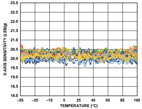
Figure 6. X-Axis Sensitivity vs. Temperature, 15 Devices Soldered to PCB, V_S = 2.5\text{ V}
