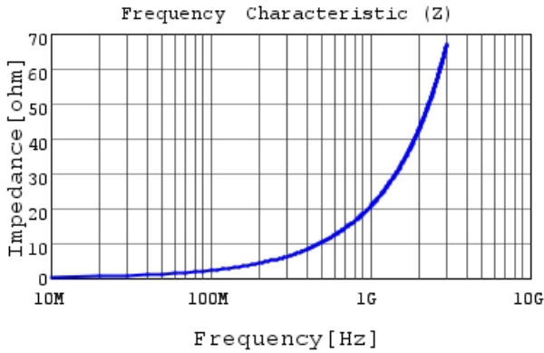
LQP03TQ3N3C02 |Z|
