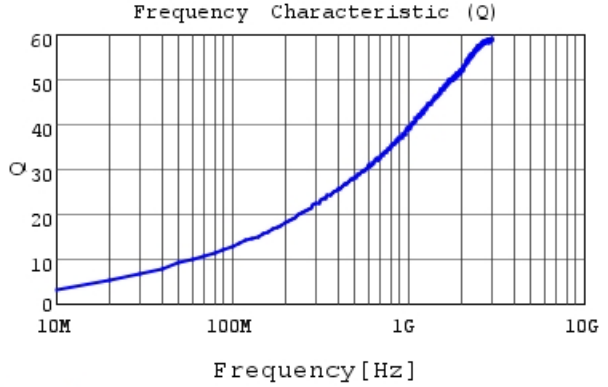
LQP03TQ3N3C02 Q
