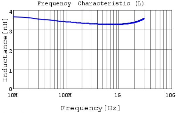
LQP03TQ3N3C02 L
