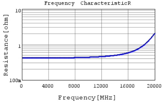
GCQ1555C1HR30BB01 R DC0V, 25degC
