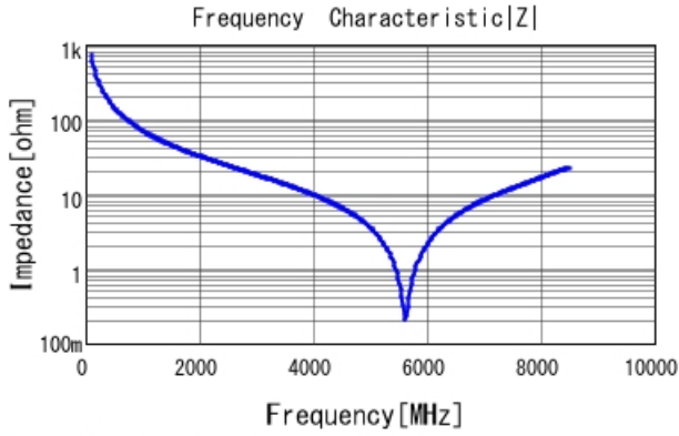
GQM1875C2E2R2CB12 |Z| DCOV, 25degC
