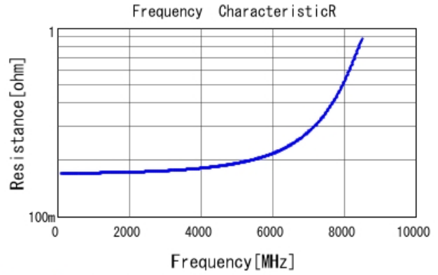
GQM1875C2E2R2CB12 R DCOV, 25degC
