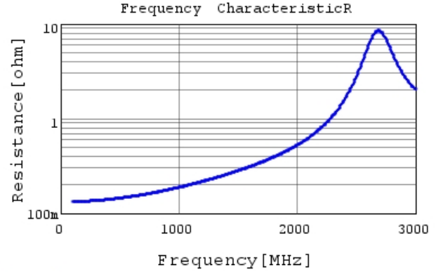
GRM31A5C3A330JW01 R DC0V, 25degC
