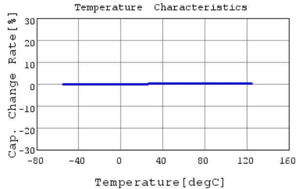
GRM31A5C3A330JW01 C-Temp. capchange, DC0V, 1
