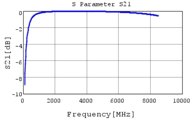
GCQ1555C1H6R1BB01 S21 DCOV, 25degC
