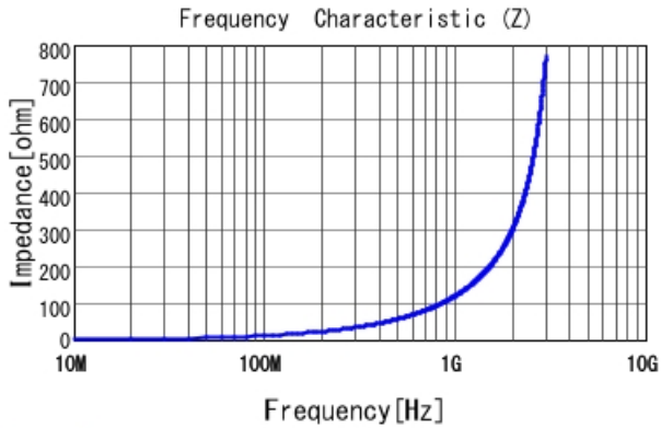
LQW2BAS18NJ00 |Z|
