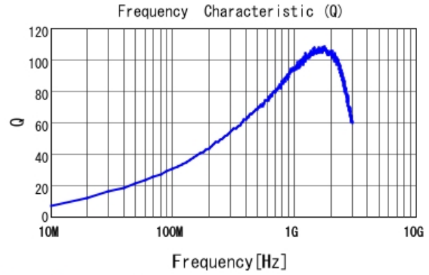
LQW2BAS18NJ00 Q
