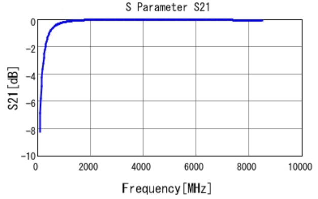
GJM0335C1E6R7BB01 S21 DC0V, 25degC
