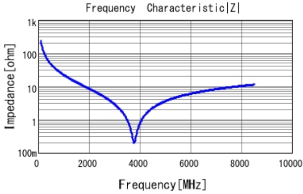
GJM0335C1E6R7BB01 |Z| DCOV, 25degC
