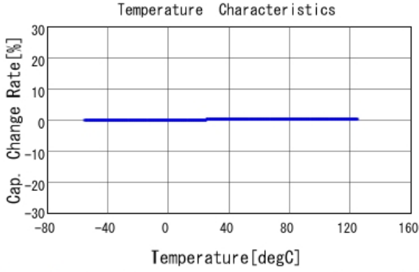
GJM0335C1E6R7BB01 C-Temp. capchange, DC0V, AC1Vrms
