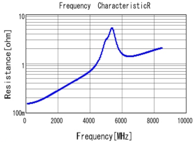
■ GRM0332C1H200JA01 R DC0V, 20degC
