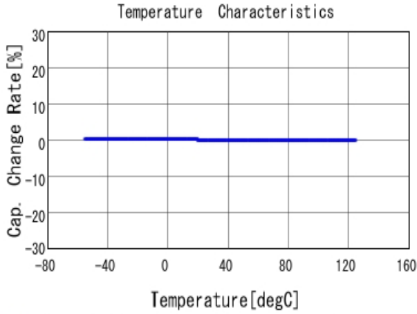
■ GRM0332C1H200JA01 C-Temp. capchange, DCOV, AC1Vrms
