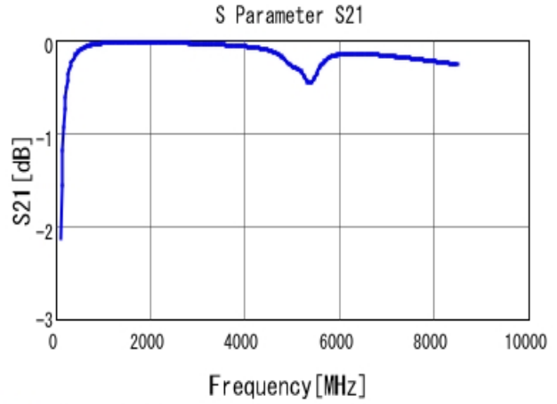
■ GRM0332C1H200JA01 S21 DCOV, 20degC
