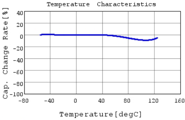
RDER71H472K0P1H03B C-Temp. capchange, DC0.0V
