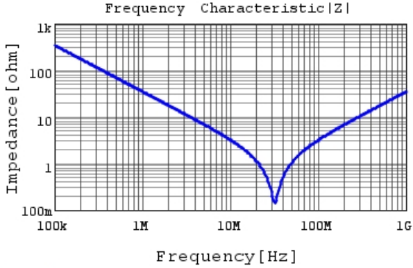
RDER71H472K0P1H03B |Z| DCOV, 25degC
