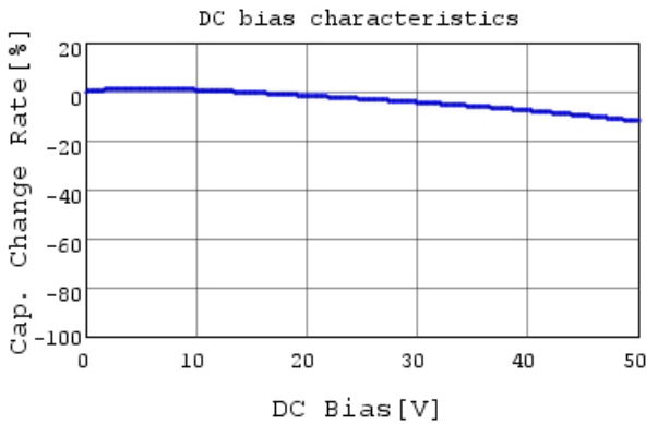
RDER71H472K0P1H03B C-DC bias capchange, 25.0
