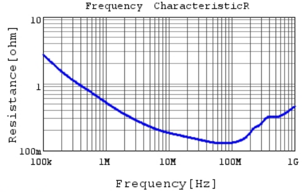
RDER71H472K0P1H03B R DCOV, 25degC
