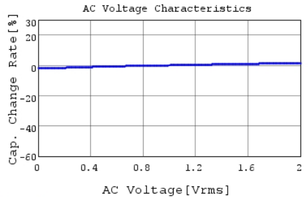
RDER71H472K0P1H03B C-AC Voltage capchange, I
