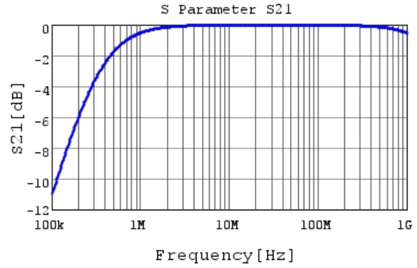
RDER71H472K0P1H03B S21 DC0V, 25degC
