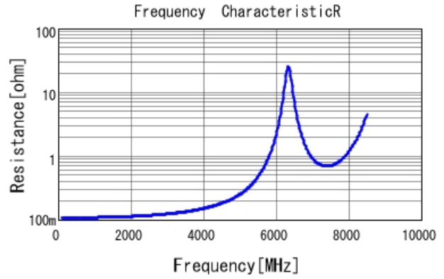
GQM1555C2D100JB01 R DCOV, 25degC
