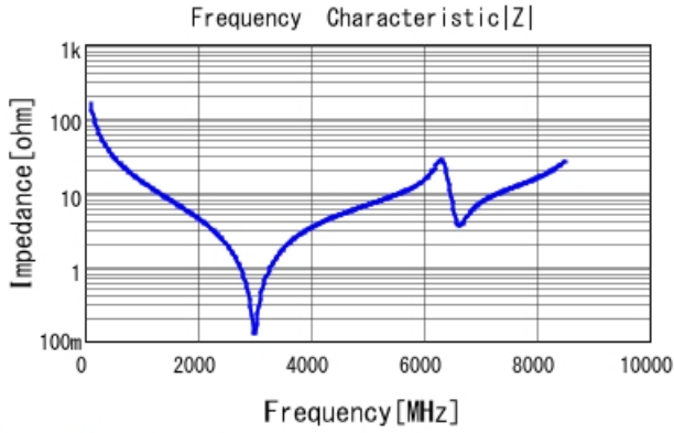
GQM1555C2D100JB01 |Z| DCOV, 25degC
