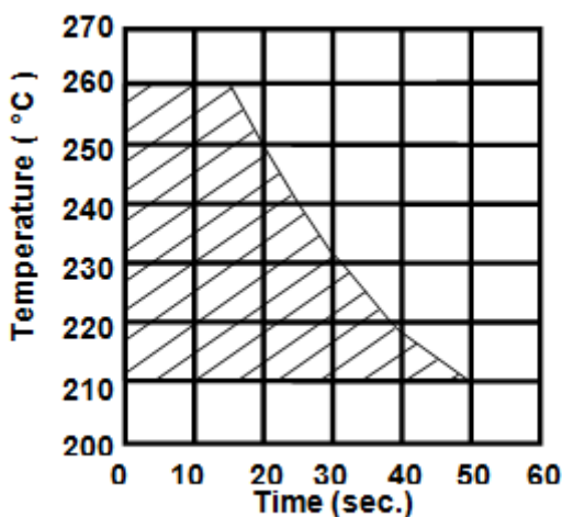
<Allowable Reflow Soldering Temp. and Time>
