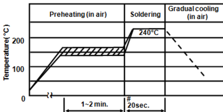
<Reflow Soldering Condition>
