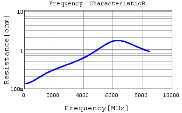
GRM0332C2A360JA01 R DCOV, 20degC
