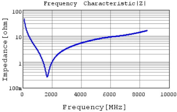
GRM0332C2A360JA01 |Z| DCOV, 20degC
