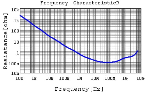
GRM033B11A472MA01 R DCOV, 20degC
