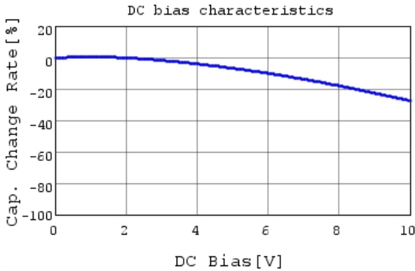
GRM033B11A472MA01 C-DC bias capchange, 20.0c
