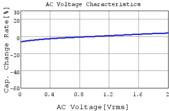
GRM033B11A472MA01 C-AC Voltage capchange, Dc
