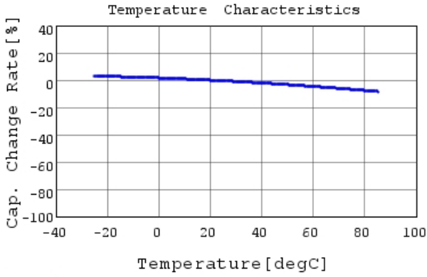
GRM033B11A472MA01 C-Temp. capchange, DC0.0V,
