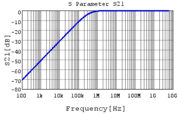
GRM033B11A472MA01 S21 DC0V,20degC
