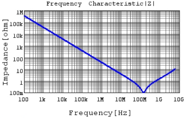
GRM033B11A472MA01 |Z| DCOV, 20degC
