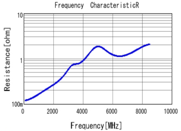
■ GRM0332C1H510JA01 R DC0V, 20degC
