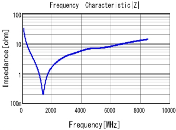
■ GRM0332C1H510JA01 |Z| DC0V, 20degC
