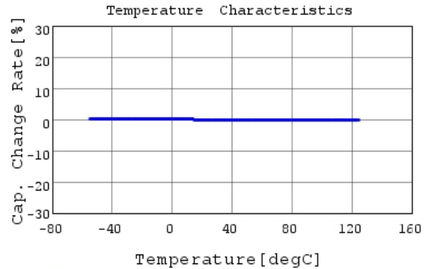
GRM1885C2E470FW07 C-Temp. capchange, DCOV, 1
