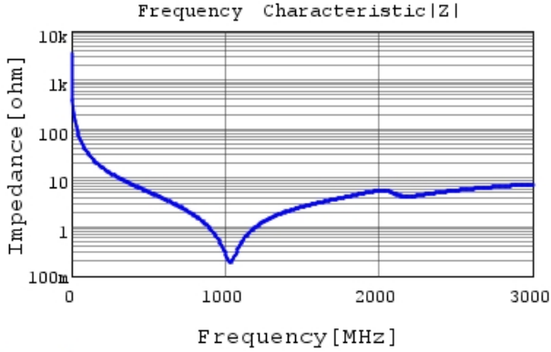
GRM1885C2E470FW07 |Z| DCOV, 25degC
