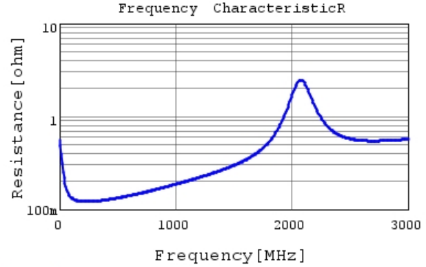
GRM1885C2E470FW07 R DCOV, 25degC
