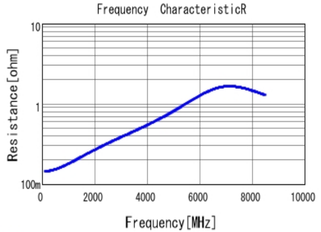
■ GRM0332C1H300JA01 R DC0V, 20degC
