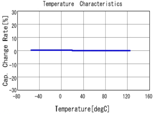
■ GRM0332C1H300JA01 C-Temp. capchange, DCOV, AC1Vrms
