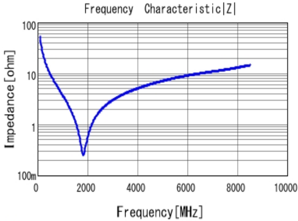
■ GRM0332C1H300JA01 |Z| DC0V, 20degC
