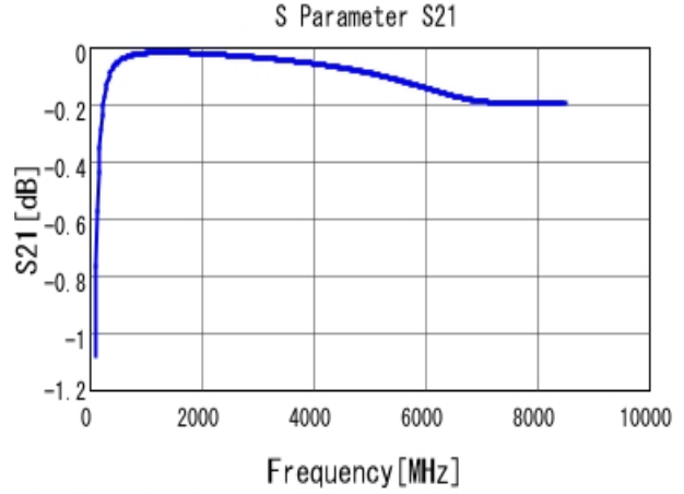
■ GRM0332C1H300JA01 S21 DCOV, 20degC
