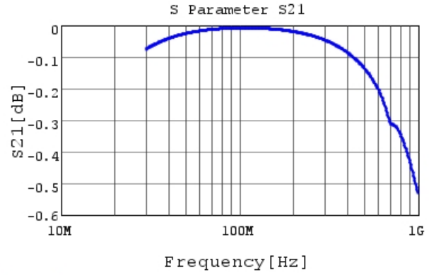
RDE5C1H391J0P1H03B S21 DCOV, 25degC
