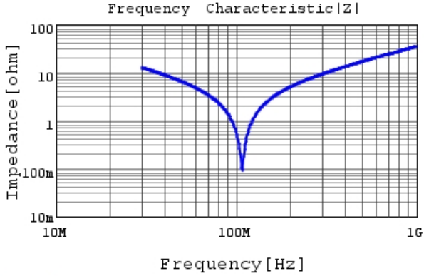
RDE5C1H391J0P1H03B |Z| DC0V, 25degC
