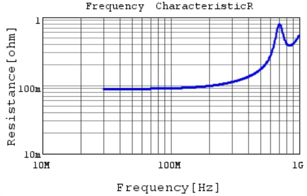
RDE5C1H391J0P1H03B R DC0V, 25degC
