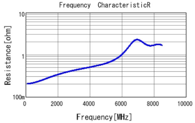
GRM1555C1H6R5CA01 R DCOV, 25degC
