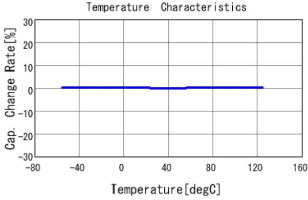
GRM1555C1H6R5CA01 C-Temp. capchange, DCOV, AC1Vrms
