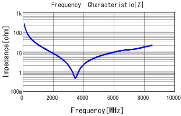
GRM1555C1H6R5CA01 |Z| DCOV, 25degC
