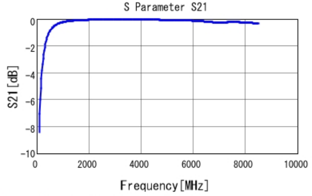
GRM1555C1H6R5CA01 S21 DCOV, 25degC
